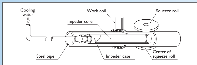
High-frequency inductive pipe welding
